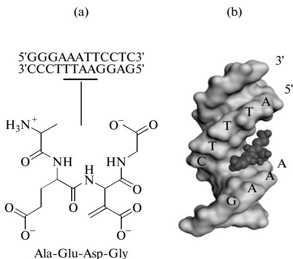
Fig. 3. Molecular model of a complementary interaction of the Ala-Glu-Asp-Gly peptide and the DNA double helix: (a) peptide structure and DNA sequence to which the peptide binds; (b) localization of the peptide in DNA major groove.
