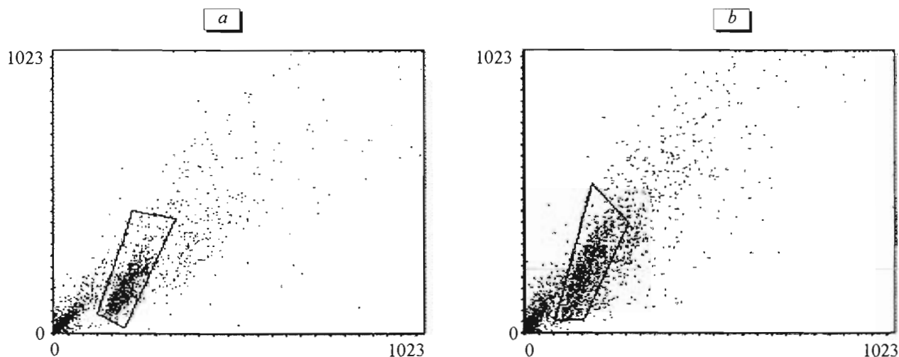
Fig. 3. Results of evaluation of telomere length by fluorescent in situ hybridization with flow cytometry (flow-FISH). Fetal fibroblasts in control (a), Epithalon-treated fetal fibroblasts (b). Vertically: telomere staining with PNA-FITC probe (linear scale). Horizontally: cell DNA staining with propidium iodide (linear scale). Cells in the G1 phase of cell cycle are in the frame.
